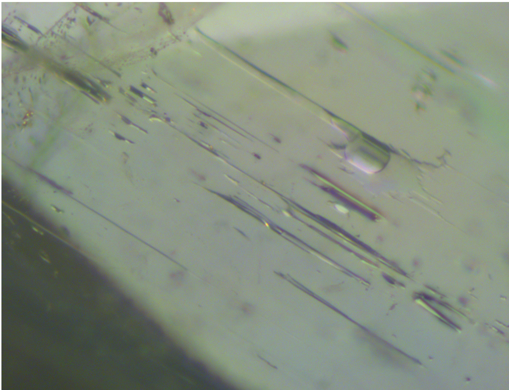
Liquid filled rain inclusions in beryl variety aquamarine
