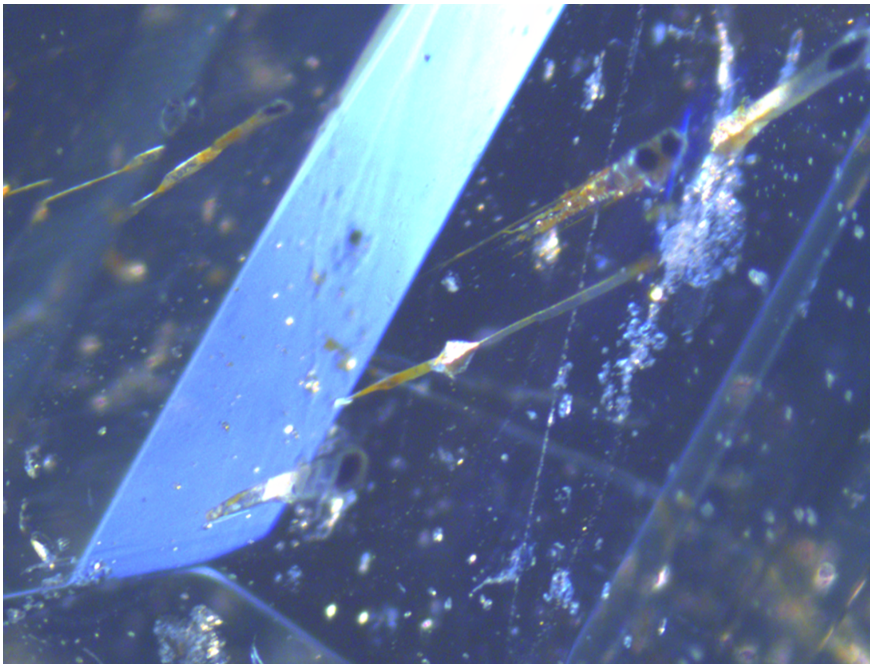
Iron-stained inclusions in beryl variety aquamarine
