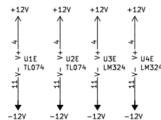
Powering the OpAmps
