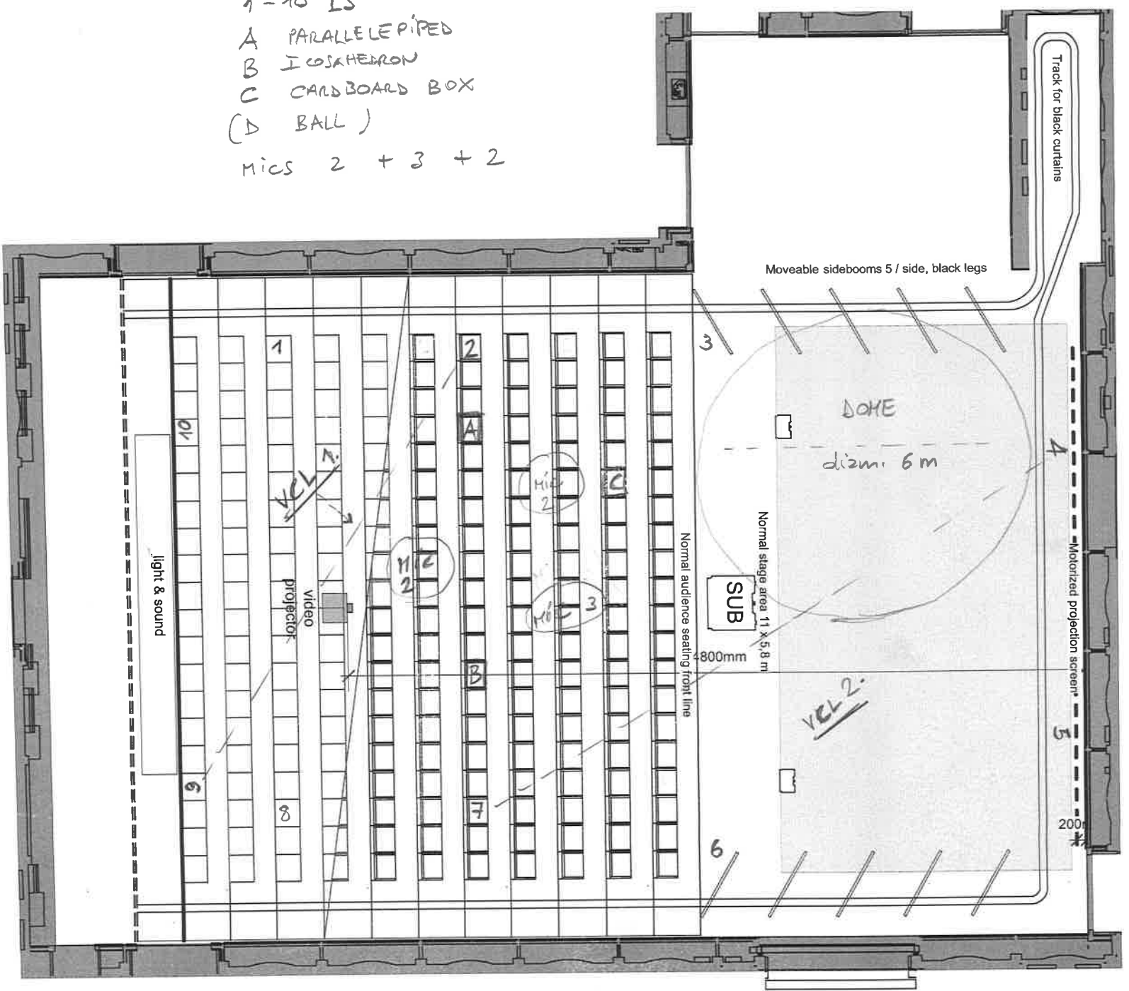
BLACK BOX STAGE PLAN
