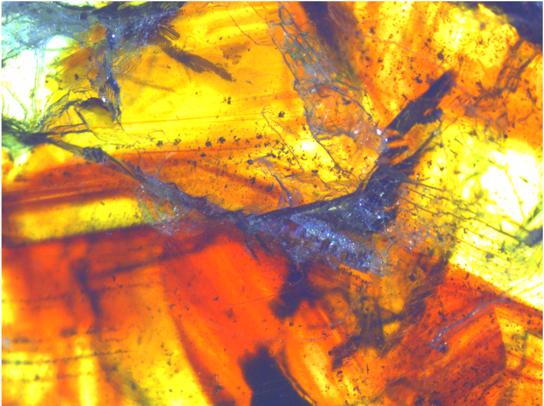
Colour zoning in sphalerite with fractures, and unknown primary inclusions
