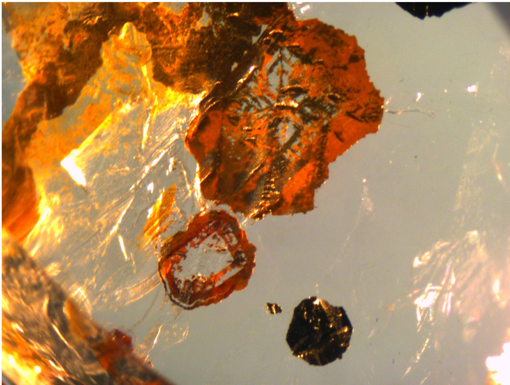
Pyrite inclusions in picture quartz
